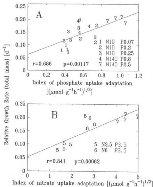
Fig. 2. Relation of relative growth rate, RGR , to index of uptake rate, \sqrt{rv/(1+r)} , predicted to be linearly related to RGR . Here, v is uptake velocity per unit root mass. Individual replicate plants in a treatment are identified with the number of that treatment; see Table 1 for treatment conditions. All data refer to final day 17 of treatment.
