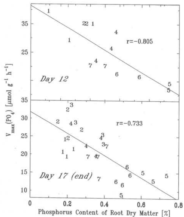
Fig. 3. Relation of V_{\text{max}} for phosphate uptake to total phosphorus content in root as fraction of dry matter. Individual replicate plants in a treatment are identified with the number of that treatment; see Table 1 for treatment conditions.
